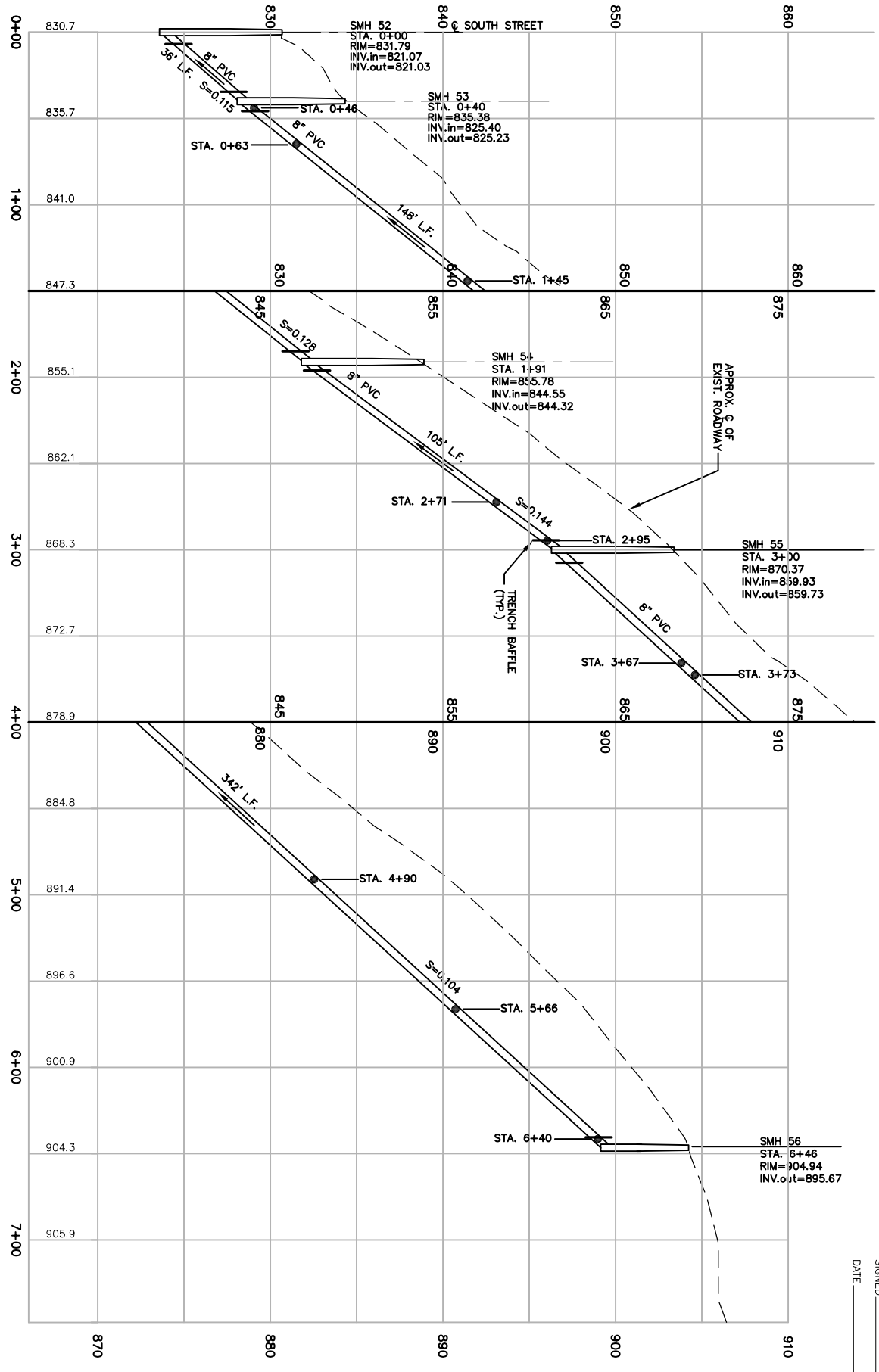
PROFILE SCALE: 1"=40' HORIZ. 1"=4' VERT.
